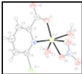
Fig. 1. ORTEP (Johnson, 1976) plot of the title compound. Displacement ellipsoids are drawn at the 50% level.
