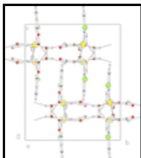
Fig. 2. Packing of the molecules in the unit cell showing the H-bonds as dashed lines.
